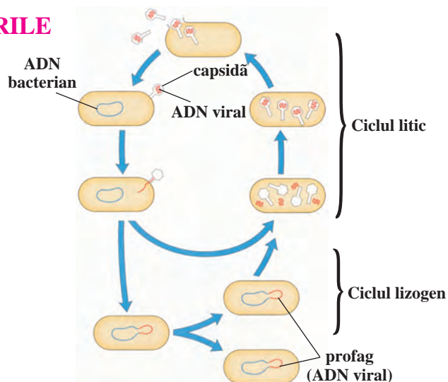
Fig. 1.4. Replicarea virusurilor
